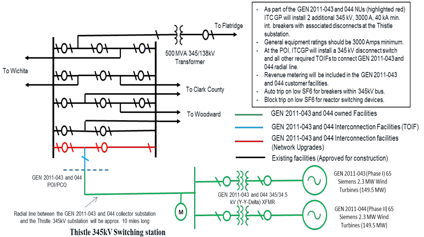
Figure 1 GEN-2011-044 ITCGP Thistle 345kV substation one line diagram
