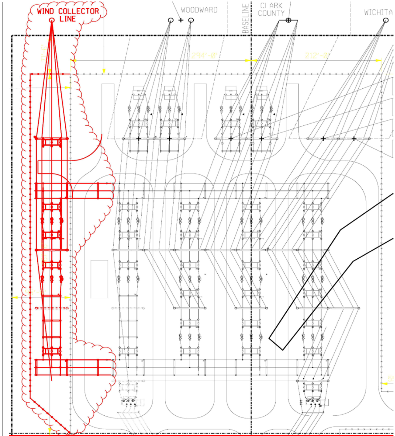
Figure 2 GEN-2011-044 ITCGP Thistle Interconnection substation site plan
